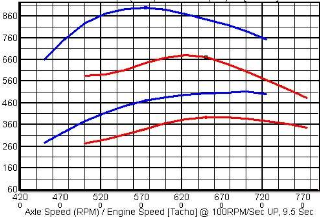
Derived Torque(FtLb) and Power(HP) [Cor'd]
